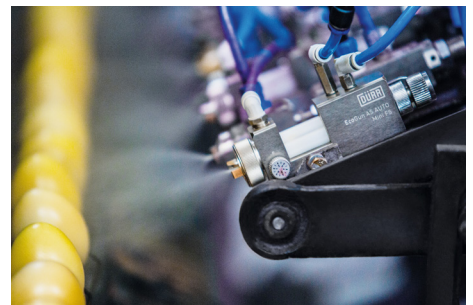
Easter egg painting using Dürr small several form factor automatic spray guns in painting line.
